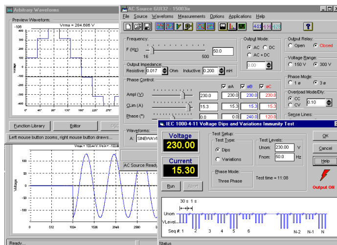
GUI application program screens for AC Source control and measurements.
